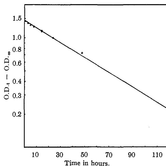
Fig. 3.—Plot of O.D. 445 - O.D. ∞ versus time to demonstrate first order reaction of the alkaline degradation of riboflavin.
