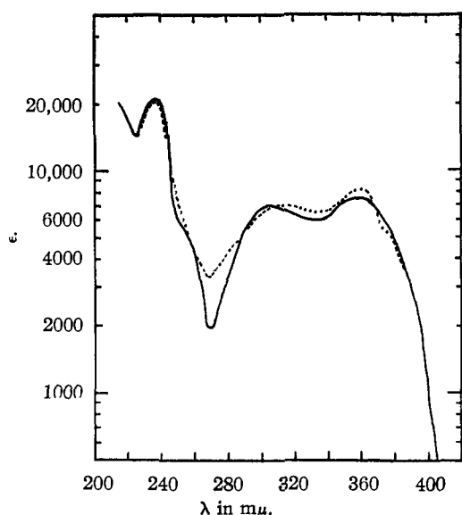
Fig. 1.— —, 3,4-Dihydro-6,7-dimethyl-3-keto-4-D-ribityl-2-quinoxalinecarboxylic acid in 0.01 N NaOH; ---, 3,4-dihydro-6,7-dimethyl-3-keto-4-methyl-2-quinoxalinecarboxylic acid in 0.1 N NaOH; redrawn (calcd. on decadic log extinction coefficients) from Kuhn and Rudy, Ber. , 67, 894 (1934).
